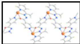
Fig. 2. A view of the zigzag chain along the a axis in (I).
